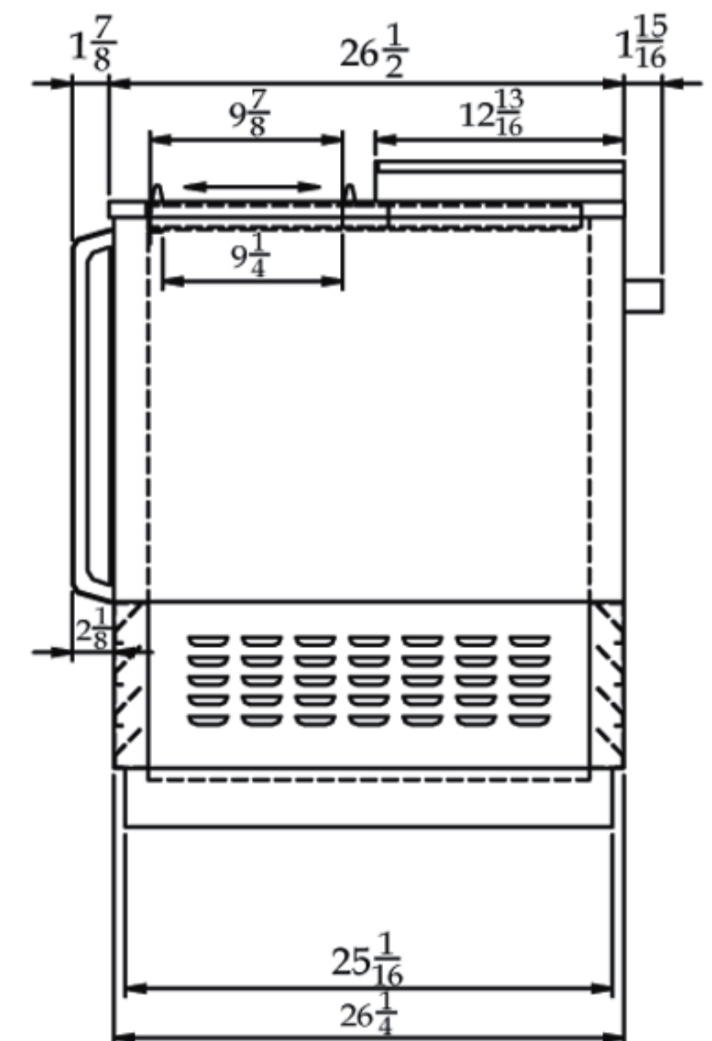
SIDE VIEW
