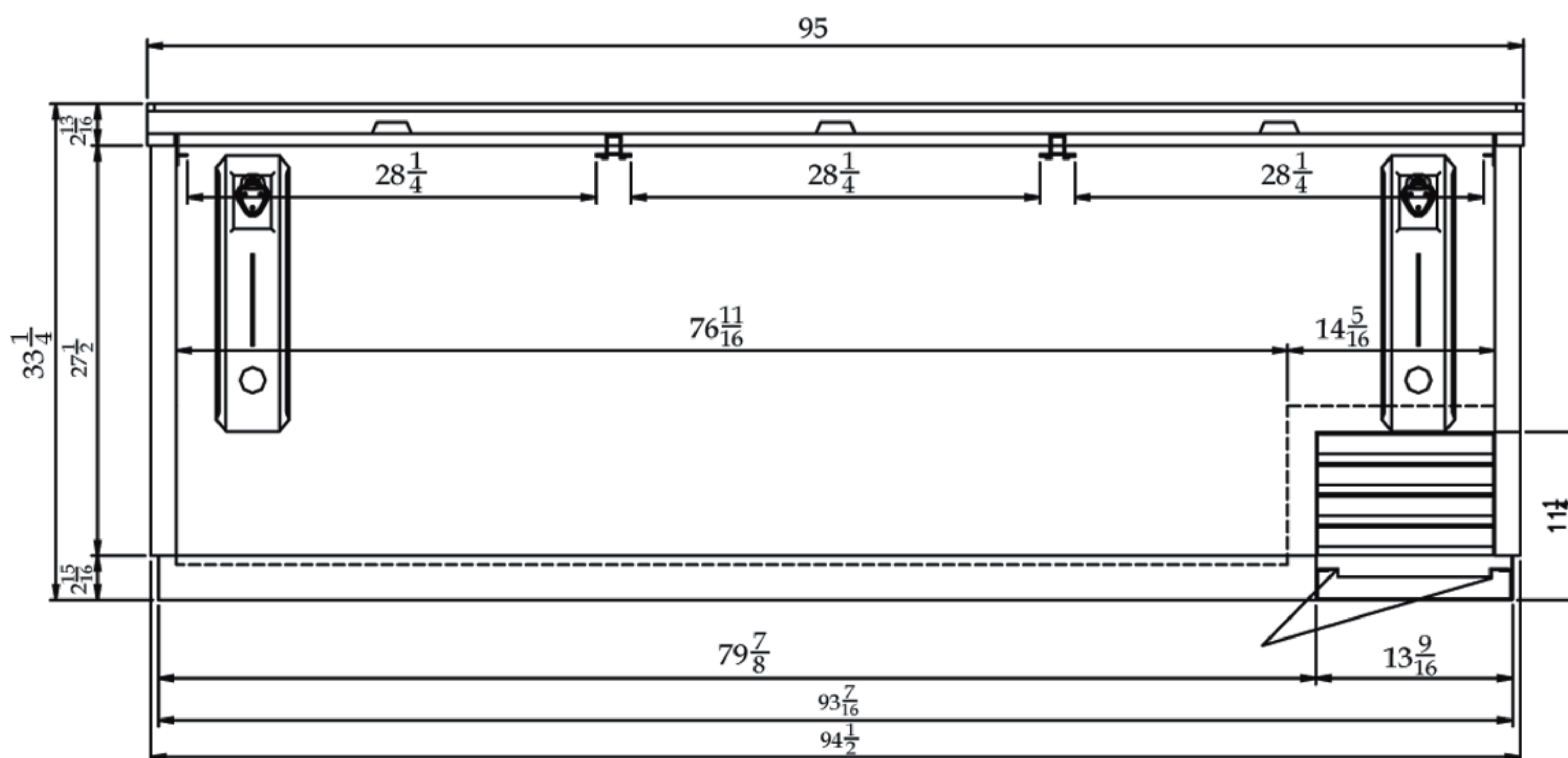
TBC-95SD/95SB FRONT VIEW
