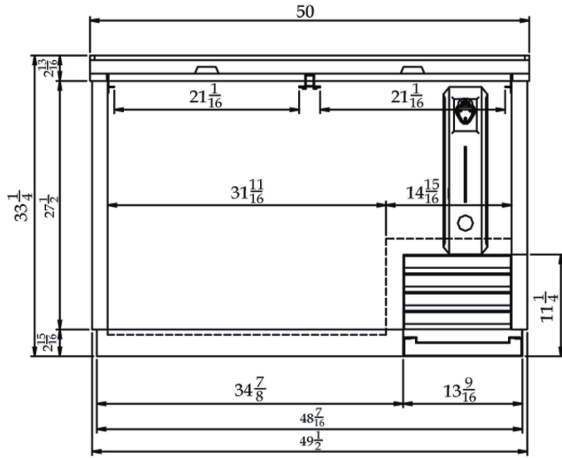
TBC-50SD/50SB FRONT VIEW
